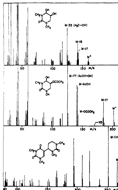
Figure 3. Mass spectra of 1,3-dimethyl- cis -4,5-dihydroxy-2-oxo-hexahydropyrimidine (IX), its 5-O-acetate (XI), and dimer III.
