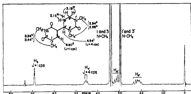
Figure 2. The nmr spectrum of dimer III in deuteriochloroform.
