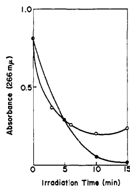
Figure 1. Heat-reversible photohydration of 1,3-dimethyluracil ( \lambda_{\max} 266 m \mu ) in aqueous solution (—●—) and photoreduction in the presence of sodium borohydride ( 10^{-4} M aqueous solution) (—○—).
